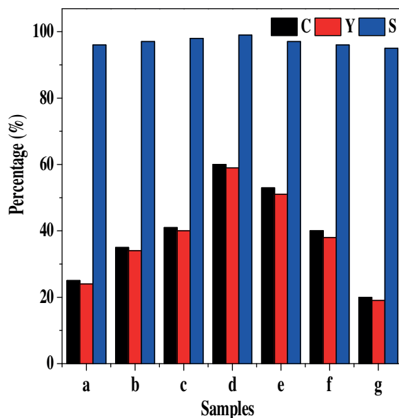
Fig. 7. Photocatalytic performance for selective oxidation of benzyl alcohol to benzaldehyde using In 2 S 3 and BN/In 2 S 3 composites under visible light irradiation for 3 h. (a) In 2 S 3 ; (b) 3% BN/ In 2 S 3 ; (c) 5% BN/ In 2 S 3 ; (d) 7% BN/ In 2 S 3 ; (e) 10% BN/ In 2 S 3 ; (f) 20% BN/ In 2 S 3 ; (g) 7% BN mixed with In 2 S 3 . (In Figs. C, Y and S mean Conversion, Yield and Selectivity, respectively.) The black, red and blue bars represent Conversion, Yield and Selectivity, respectively.) (For interpretation of the references to colour in this figure legend, the reader is referred to the web version of this article.)
