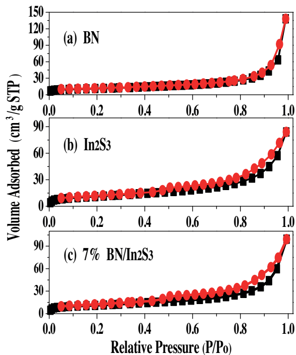
Fig. 6. Nitrogen adsorption–desorption isotherms of (a) BN, (b) In 2 S 3 and (c) 7% BN/In 2 S 3 .
