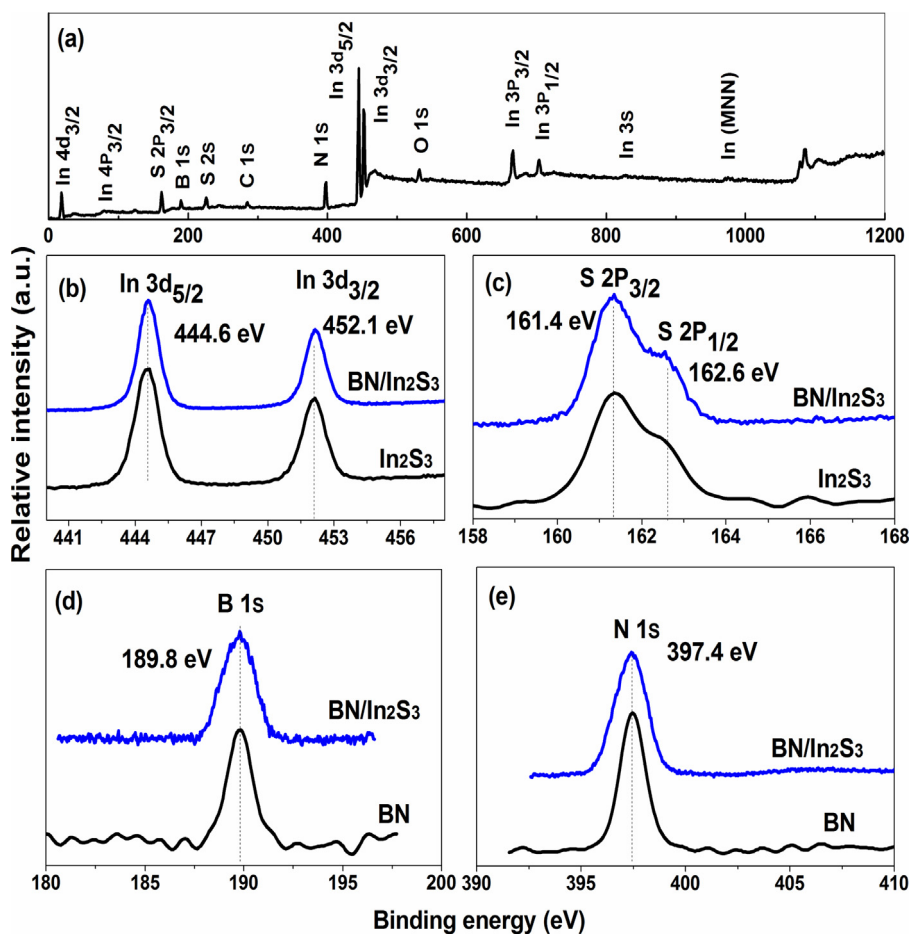
Fig. 5. (a) XPS survey spectra of 7% BN/In 2 S 3 composite. High-resolution spectra of (b) In 3d and (c) S 2p for In 2 S 3 and 7% BN/In 2 S 3 samples, and (d) B 1s and (e) N 1s for BN and 7% BN/In 2 S 3 samples.
